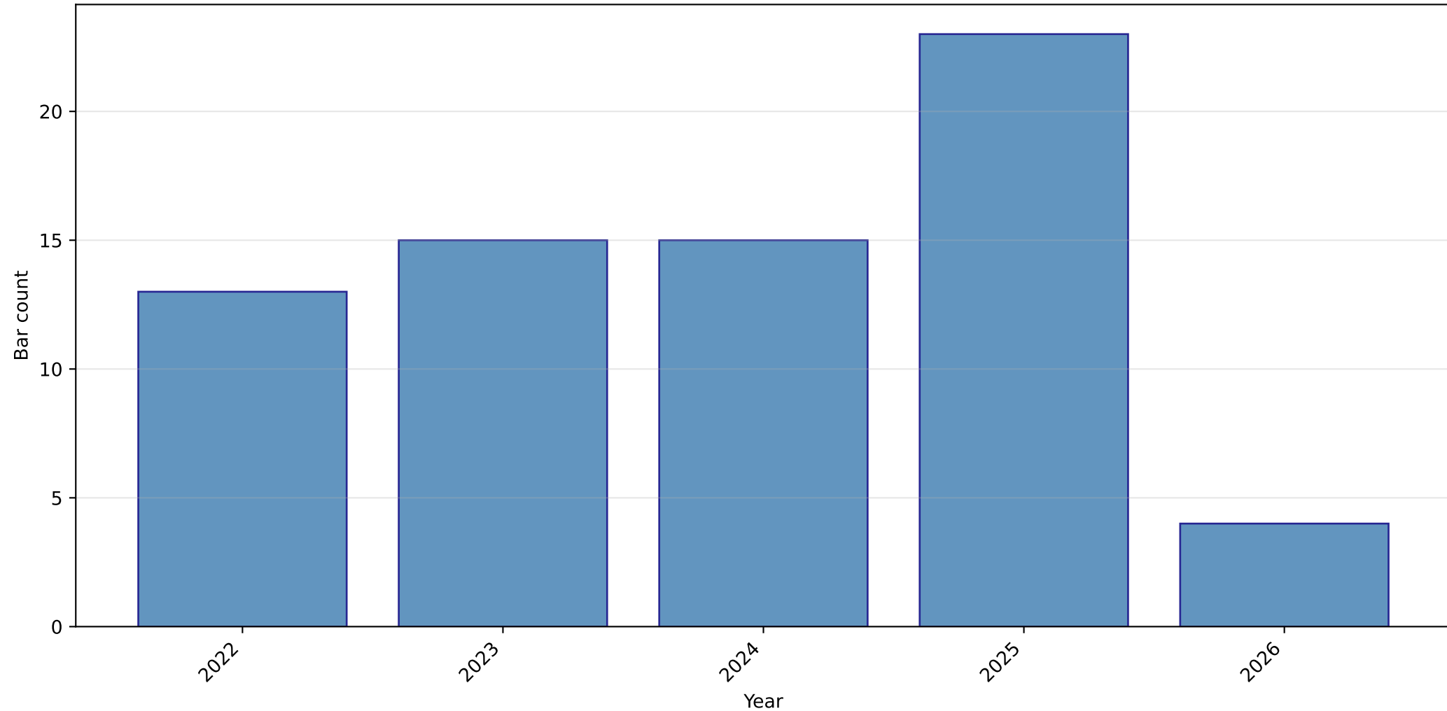
Regime 36 — bar counts by year (UTC) EURUSD · 60-minute bars (H1) · n=25,000 bars
