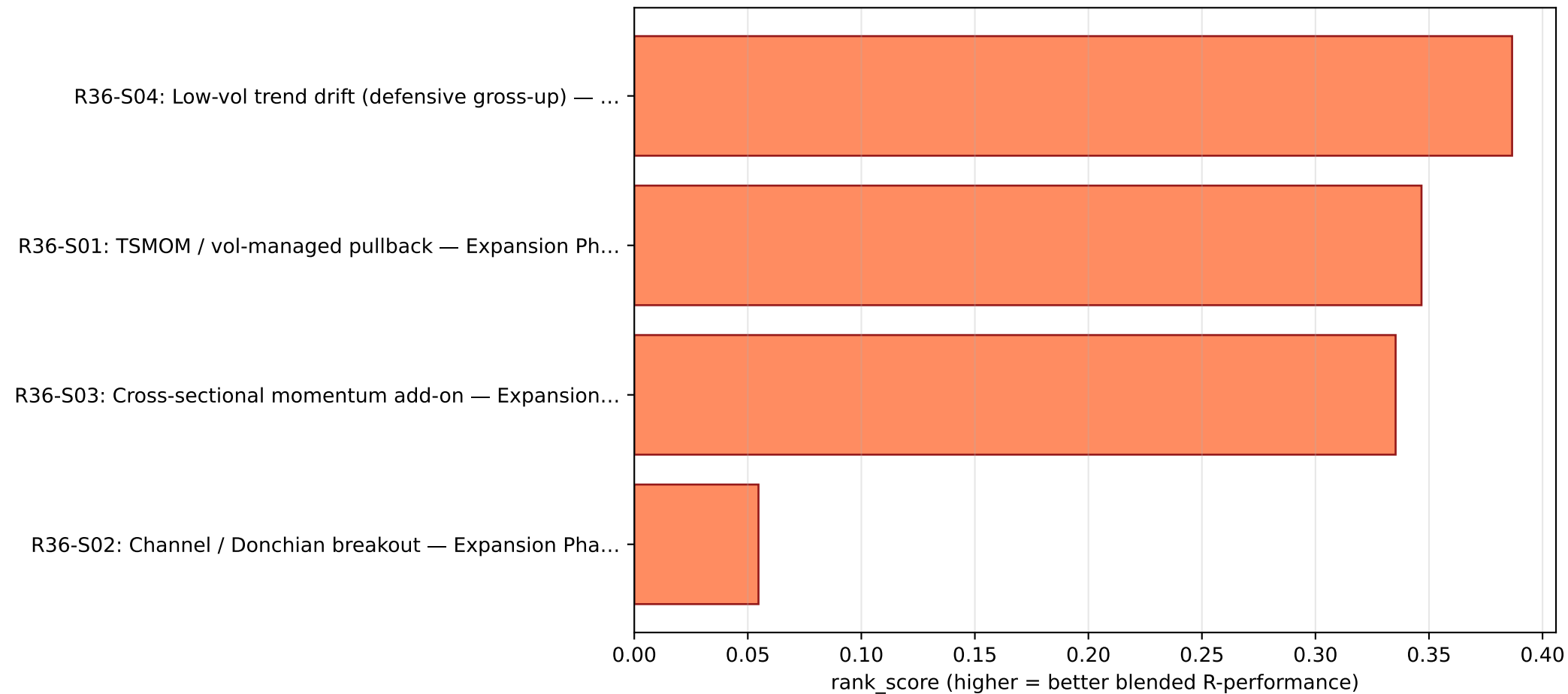
Top strategies by rank_score — regime 36 EURUSD · 60-minute bars (H1) · n=25,000 bars
